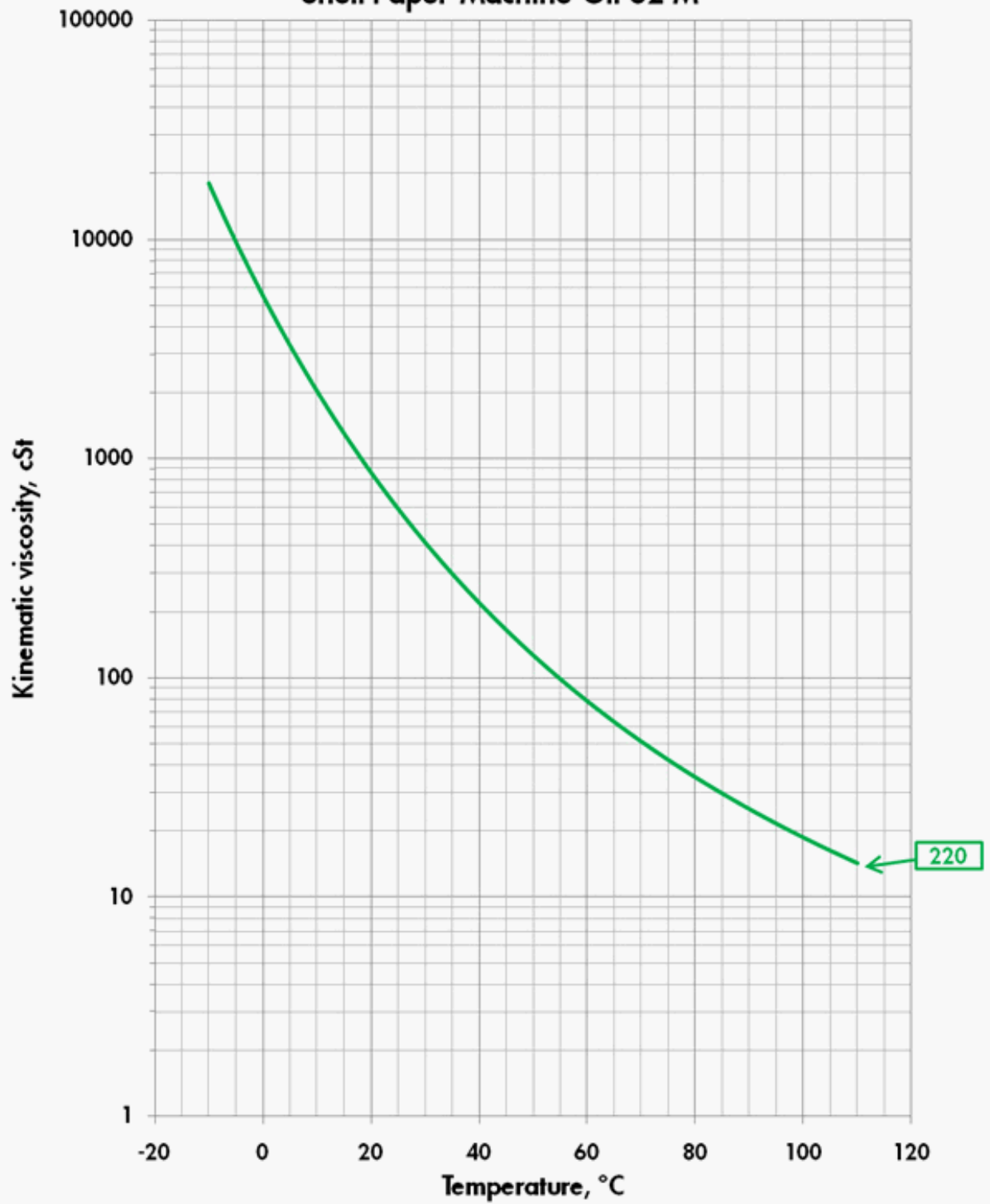
Viscosity - Temperature Diagram for Shell Paper Machine Oil S2 M
